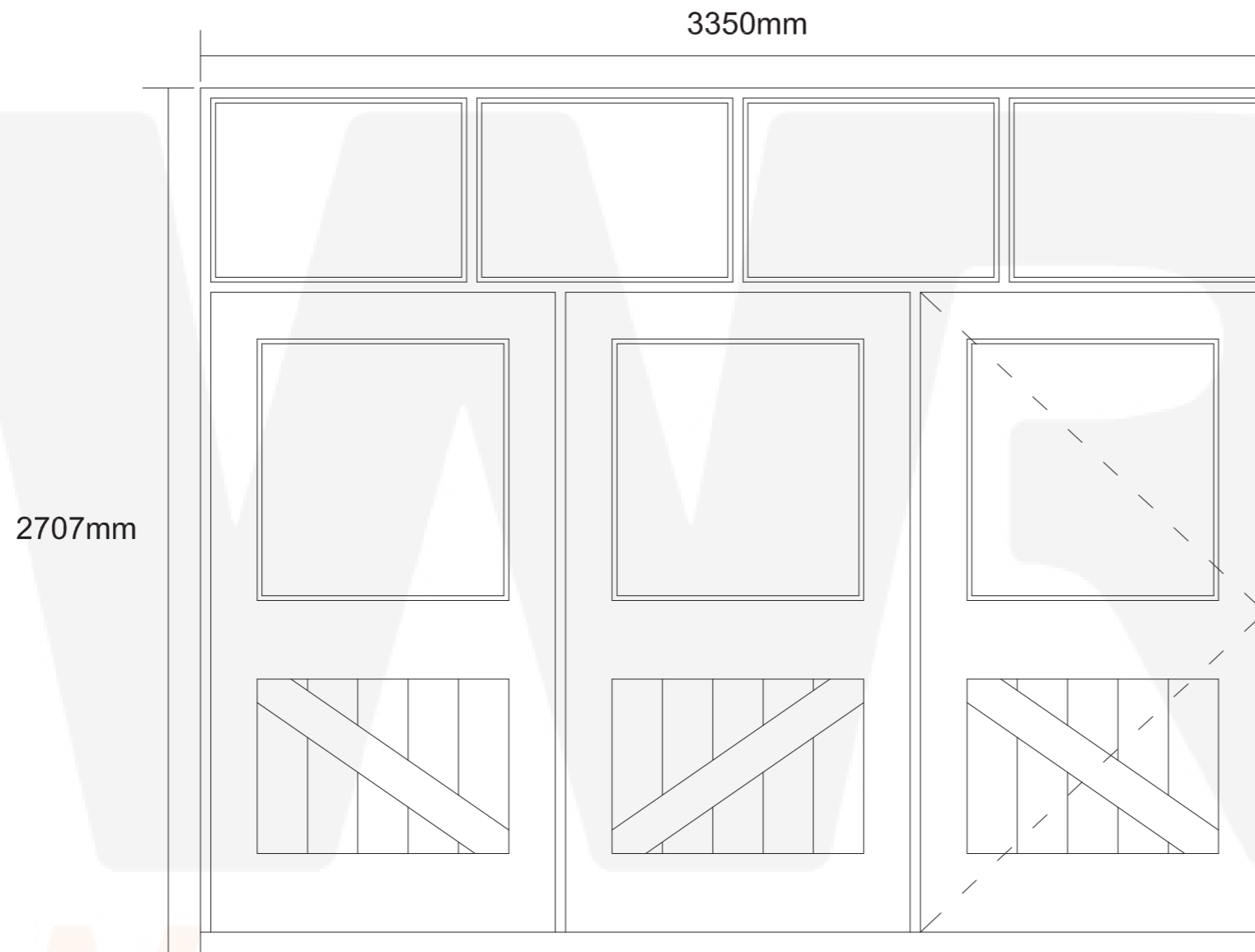
First Floor Internal - 24mm Pyrodur DG Units
