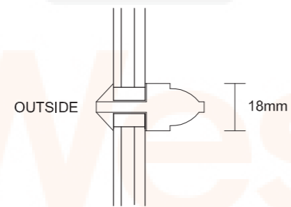
Section Through Glazing Bar
